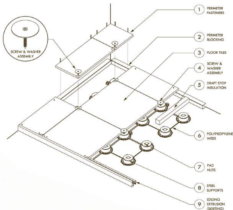
FIGURE 1a – FLOOR SYSTEM (Web Design Version #1)
